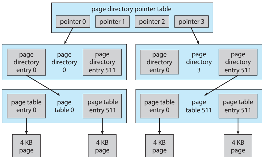
Figure 21.3 Page-table layout.
