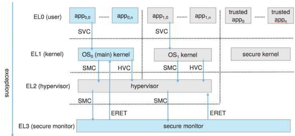
Figure 17.3 ARM architecture.
