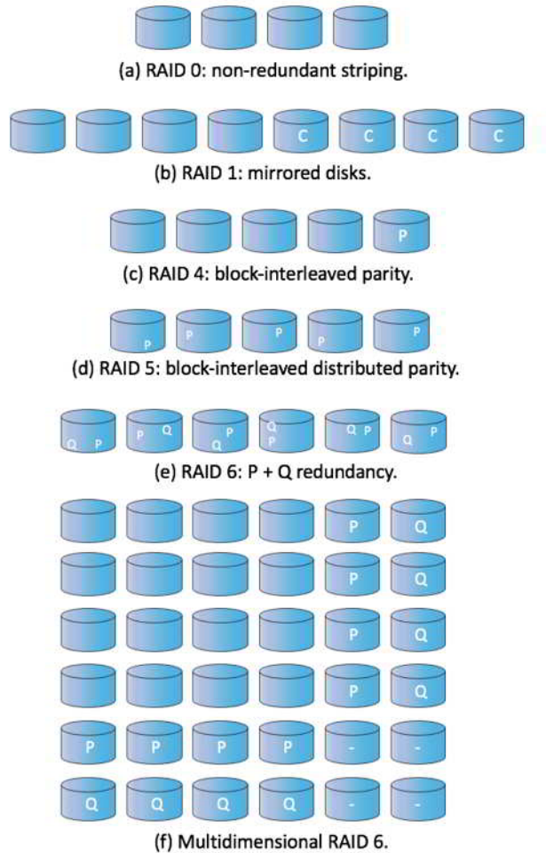
Figure 11.15 RAID levels.
