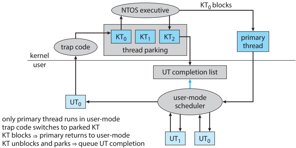
Figure 21.10 User-mode scheduling.
